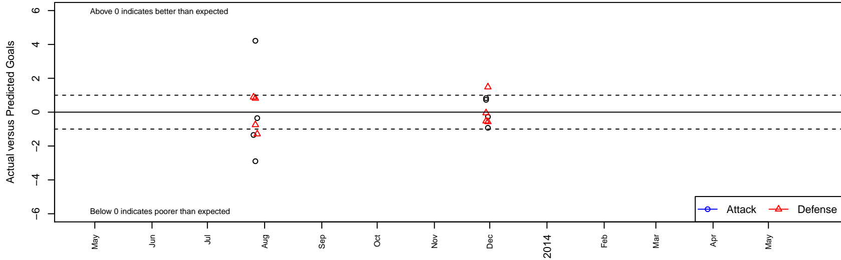
Davis Legacy Milan G99 Dots are actual minus expected GF (blue circles) and GA (red triangles). Blue line is smoothed change in attack strength. Red is smoothed change in defense strength.
